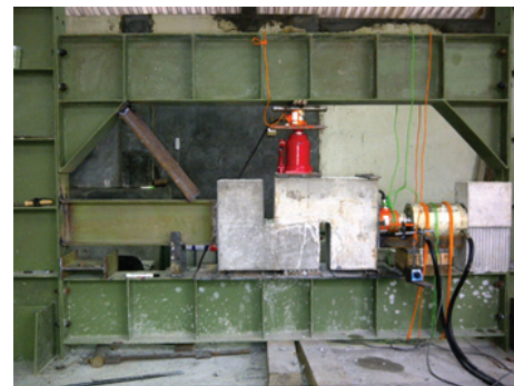
FIGURE 5: Double L-shaped shear test.
