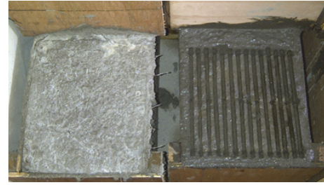
FIGURE 1: Difference of substrate surface conditions between being as-placed and grooved with 6 mm of roughness amplitude.
